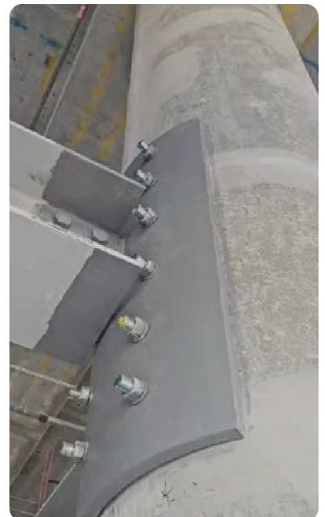
STEEL CONNECTION DETAIL
